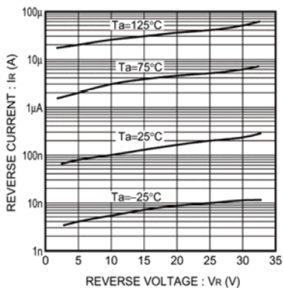
Fig. 2 Reverse characteristics
